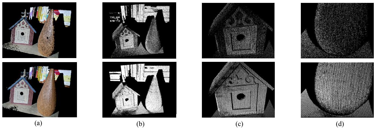
Figure 9. Objects Scene Point Clouds. a) Point-based rendering of the scene. b-d) Several views of the reconstructed point clouds. The first row are the results using standard method 2 and the second row are the results using our method.
