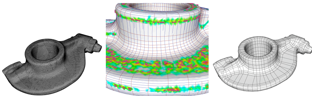
Figure 10.3: Quad-dominant remeshing. Left: The input is a manifold triangle mesh. Middle: In regions of low confidence, the curvature lines are not well-defined. The algorithm bridges these regions by extrapolation and produces the result on the right.
