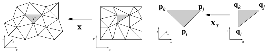
Figure 8.1: Example of a piecewise linear mapping. The meshes share the same connectivity, and individual triangles are mapped.
