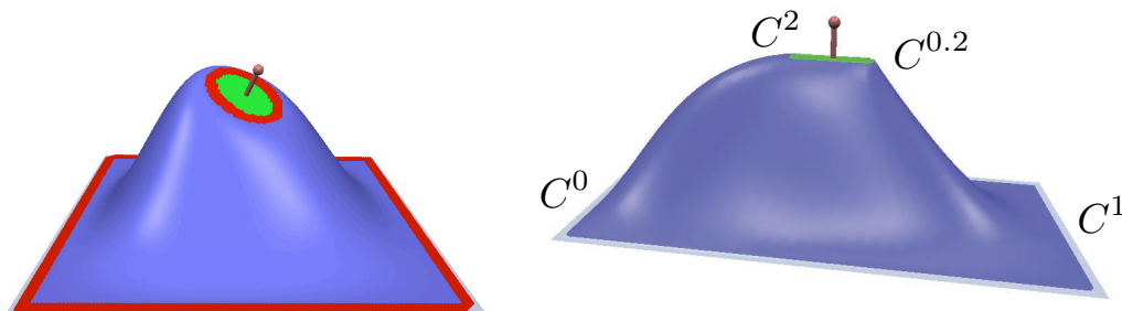
Figure 11.4: Minimizing the thin-plate energy allows for C^1 boundary constraints, which are given by the first two rings of fixed and handle vertices ( left ). The framework even allows for anisotropic bending behavior and per-vertex control of boundary continuity ( right ).
