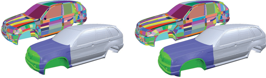
Figure 11.7: Using multiple independent handle components allows to stretch the hood while rigidly preserving the shape of the wheel houses. This 3M triangle model consists of 10k individual connected components, which are neither two-manifold nor consistently oriented.
