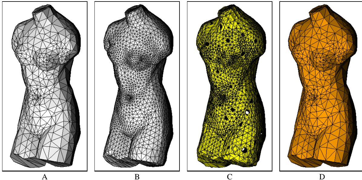
Figure 1: Algorithm overview. A: Coarse mesh ( V = 711, F = 1418, V - E + F = 2 ). B: Quadrisectioned mesh ( V = 2838, F = 5672, V - E + F = 2 ). The covering mesh of this quadrisectioned mesh has two connected components. C: First component of covering mesh ( V = 2127, F = 4254, V - E + F = -1368 ). Note the large number of holes and face overlap. D: Second component of clustering mesh equivalent to coarse mesh.
