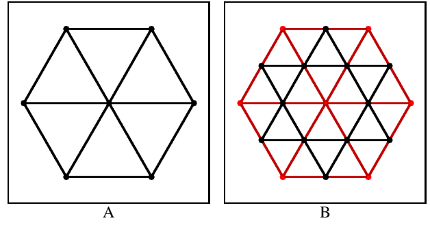
Figure 5: Example of triangle mesh quadrisection. A: coarse mesh; B: quadrisected mesh with V -vertices (red) corresponding to vertices of the coarse mesh, and E -vertices (black).
