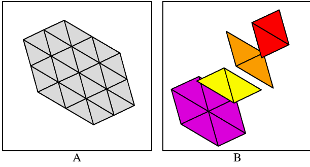
Figure 3: The covering mesh of a triangular mesh. A: quadrisected mesh. B: covering mesh with color-coded connected components. The connected components are artificially displaced in space. The quadrisection of the purple connected component is equivalent to the input mesh.
