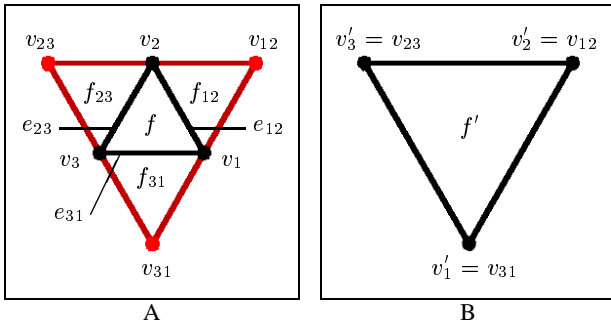
Figure 6: Notation used for tile construction. A: A tile set. B: The corresponding tile.
