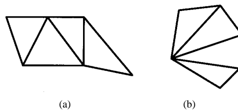
Fig. 4. (a) Triangle strip. (b) Triangle fan.
