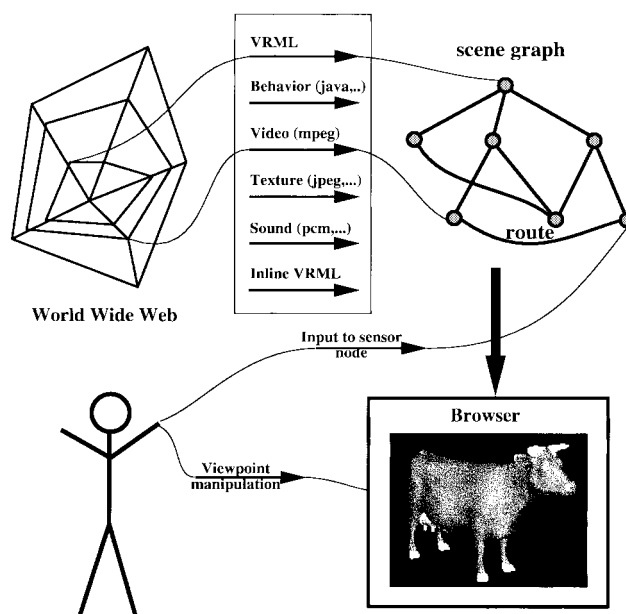
Fig. 3. Flow of information while processing a VRML file.
