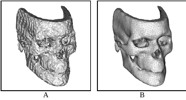
Figure 6: Effect of post-smoothing. A: Coordinates quantized to 6 bits per coordinate. B: Result of applying the smoothing algorithm of Taubin [18] with parameters n = 16 \lambda = 0.60 \mu = -0.64 . Compare with the original in Figure 8-D.
